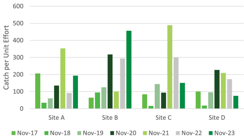
Figure 7-3. Fall Fish Survey Catch Per Unit Effort
