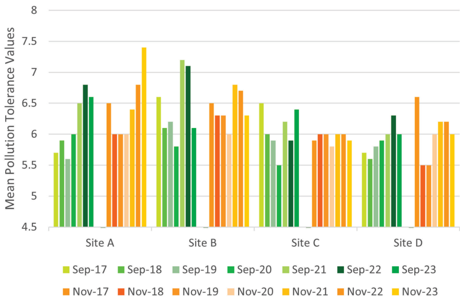
Figure 7-8. Mean Pollution Tolerance Value by Site and Sampling Date
