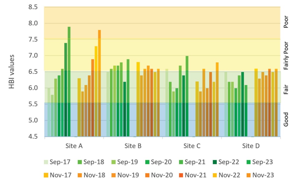
Figure 7-7. Hilsenhoff Biotic Index – Bar Graph by Site and Sampling Date
