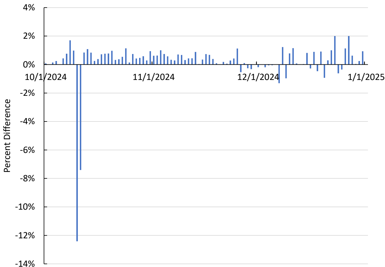
Figure 2. Percent difference between the USGS and CWP daily volume in October through December 2024. A positive value indicates USGS flow measurement is greater than the CWP's measurement.
