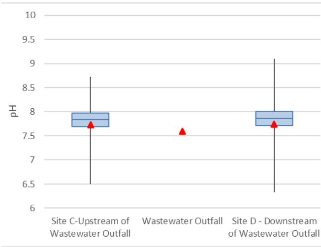
Figure 8 Plot compares the pH concentrations from the pre-diversion period (blue) to the current period (red).
