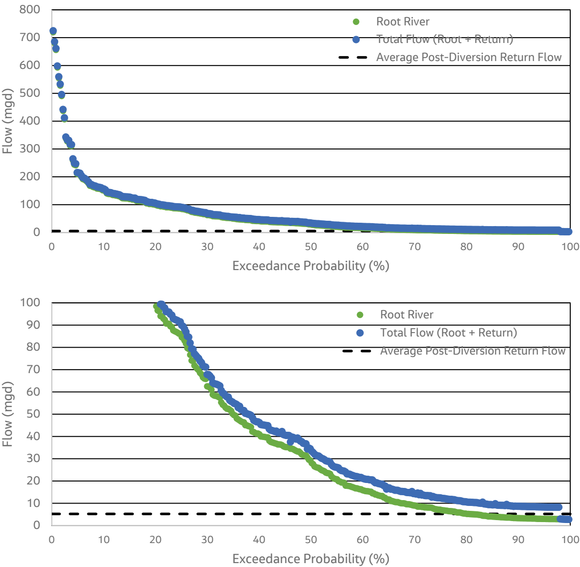
Figure 2-1. Flow Duration Curve of Daily Root River Flow and Total Flow (Root + Return)
