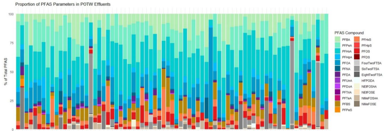
PFAS in POTW effluent expressed as a percent of total PFAS. POTWs are sorted from no SIU contributions (left) to greatest percent of influent flow from SIUs (right)
