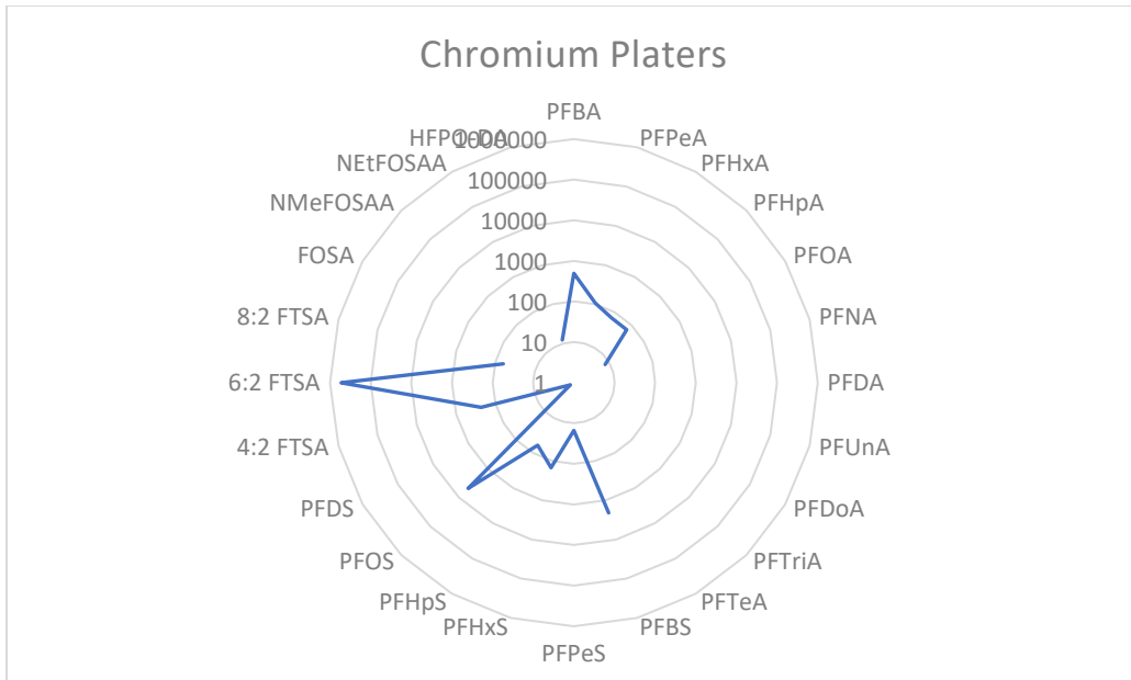
Data on PFAS in wastewater from chromium electroplaters from EPA’s Multi-Industry PFAS Study (2021)
