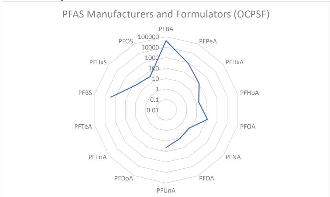
Data on wastewater concentrations of PFAS from PFAS manufacturers and formulators from EPA’s Multi-Industry PFAS Study (2021)
