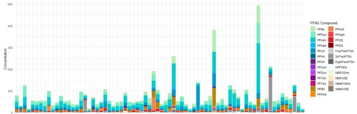
PFAS concentrations in POTW effluents, excluding one outlier POTW
