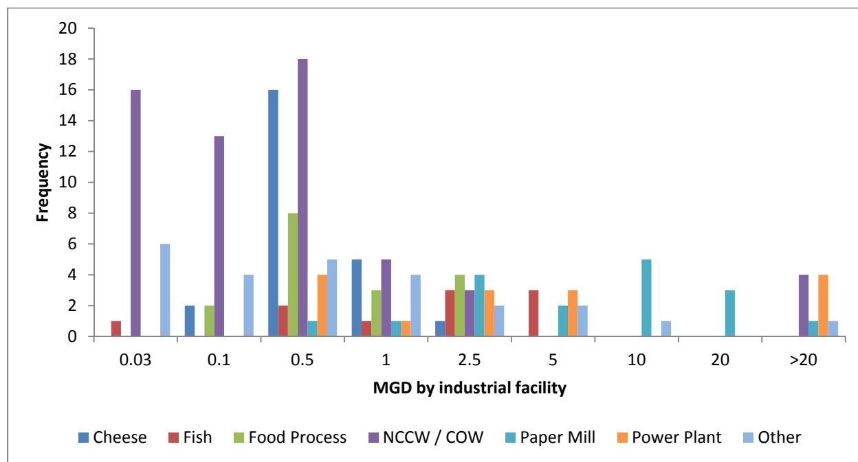
Figure 2-3 – Histogram of Industrial Facilities Based on Type of Industry and Design Flow
