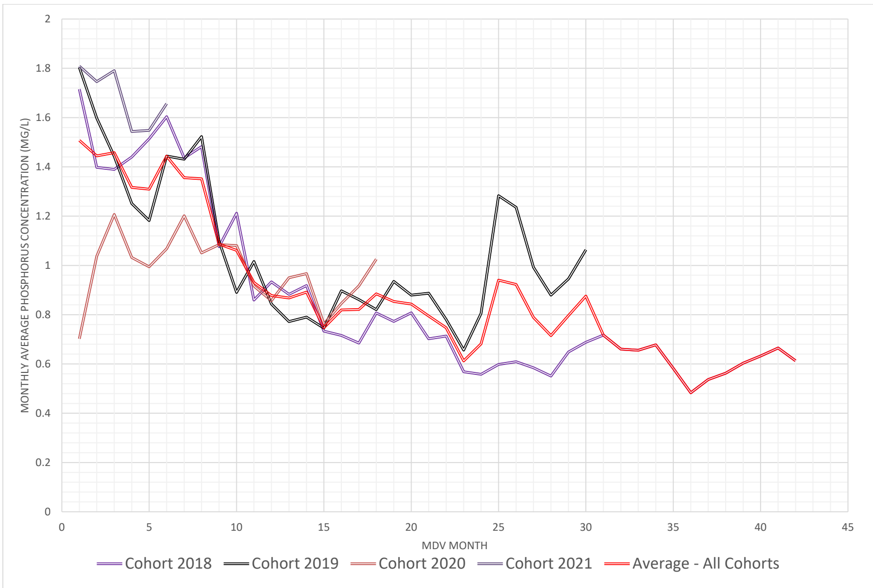
Figure: Monthly Effluent Total Phosphorus Data for all Dischargers Covered Under the MDV
