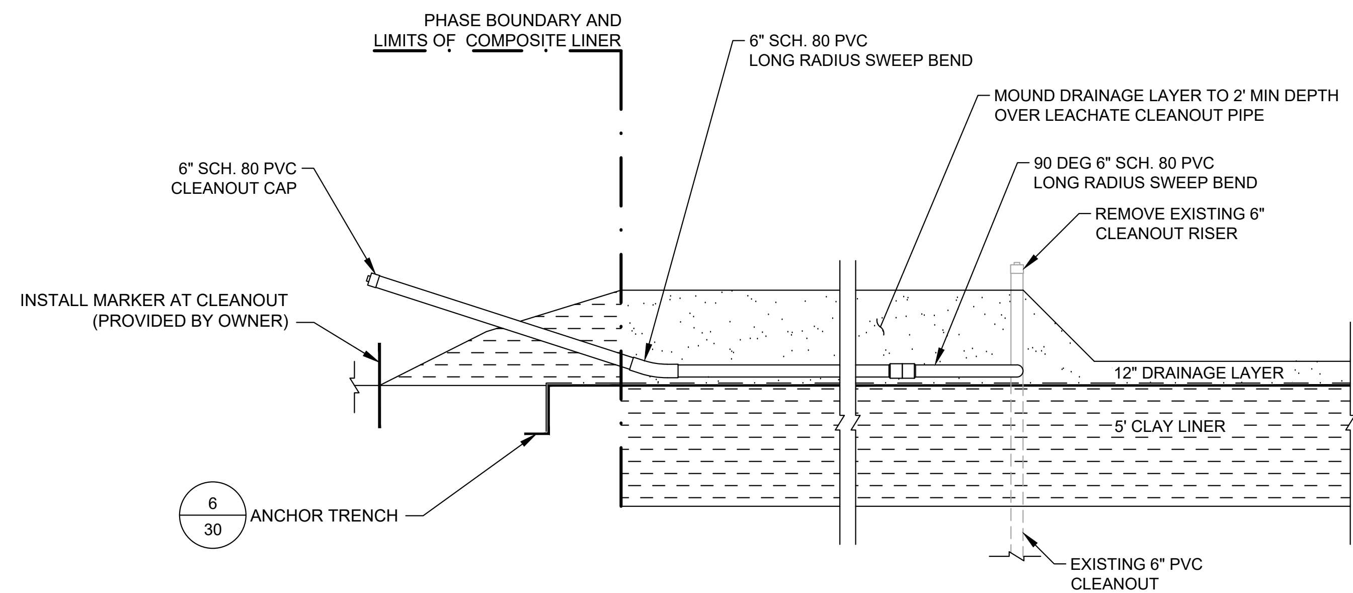
2 33 LEACHATE CLEANOUT EXTENSION - CROSS SECTION NO SCALE
