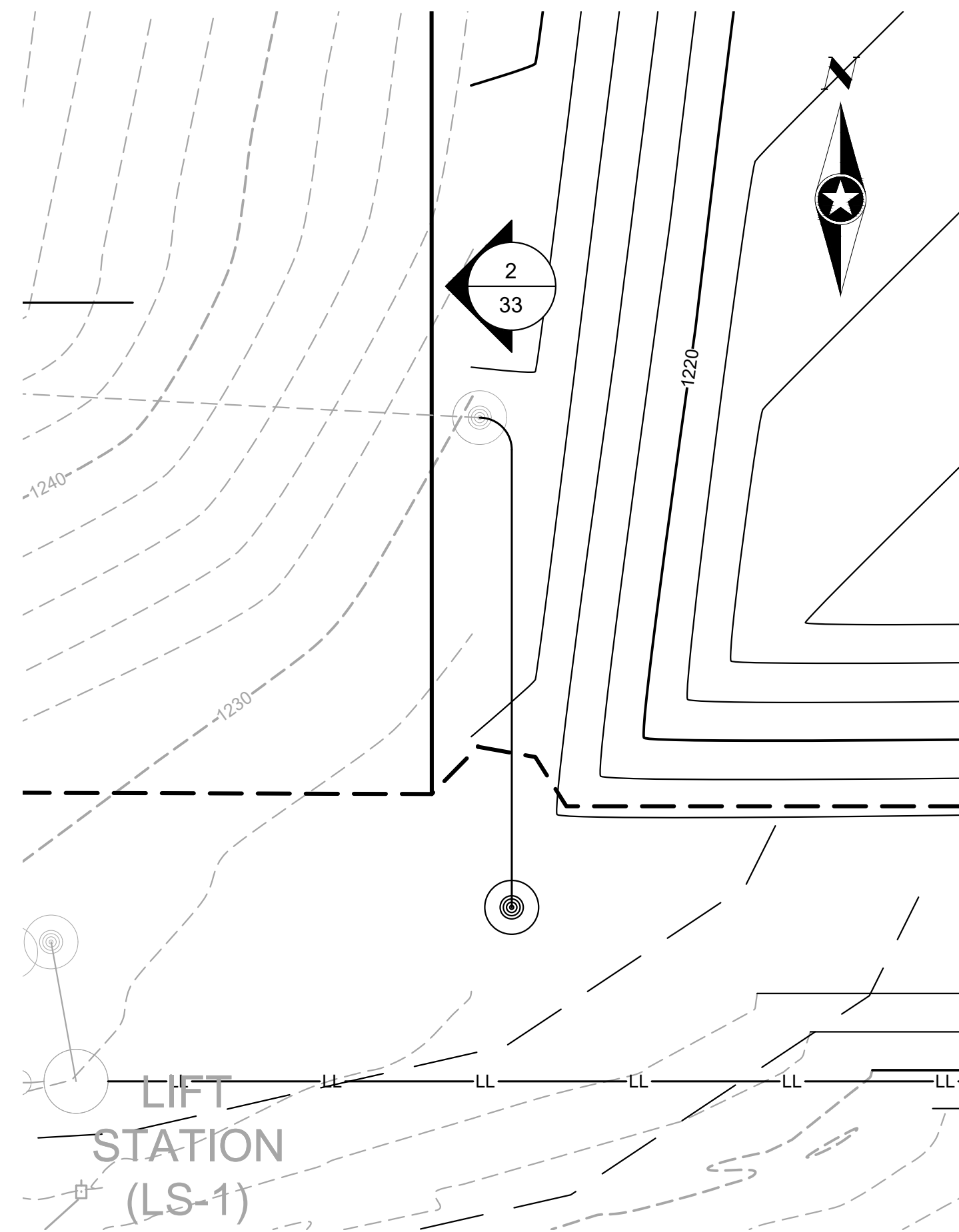
1 33 LEACHATE CLEANOUT EXTENSION - PLAN NO SCALE
