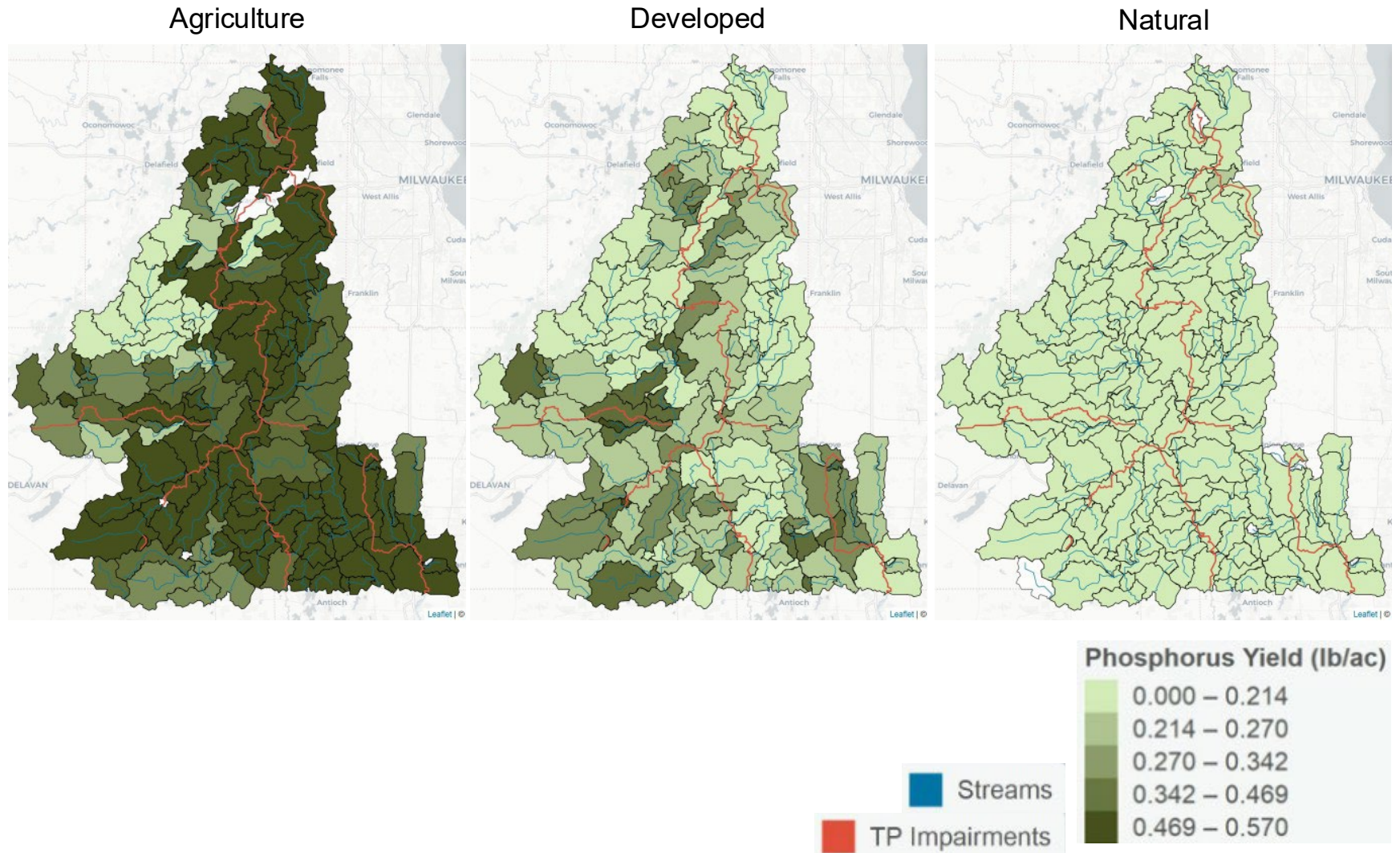
FIGURE I.16 Spatial Distribution of Average Phosphorus Yield by Land Use Categories
