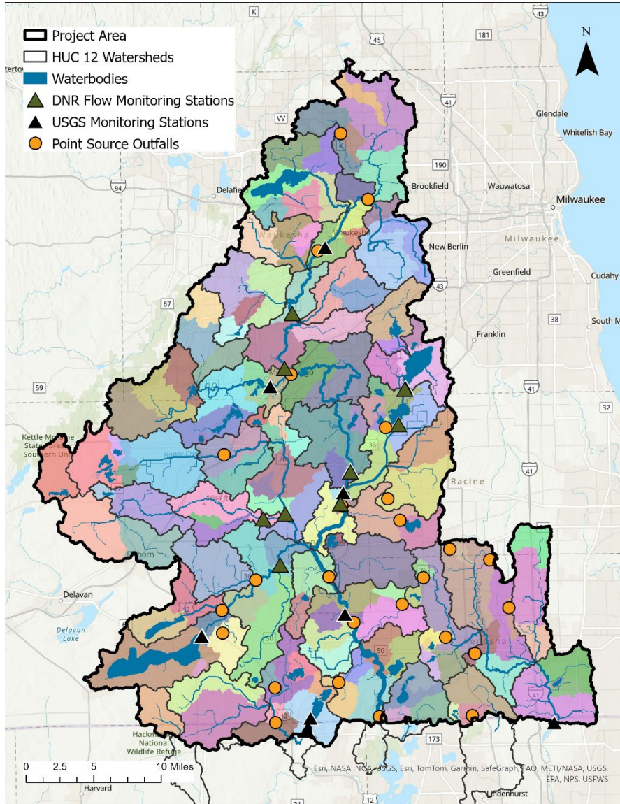
FIGURE 2.1 Final Delineation of SWAT+ Model Subbasins
