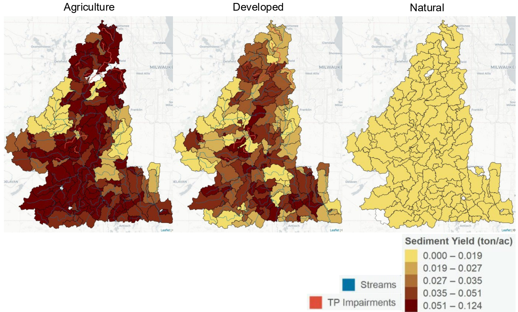
FIGURE I.7 Spatial Distribution of Average Sediment Yield by Land Use Categories
