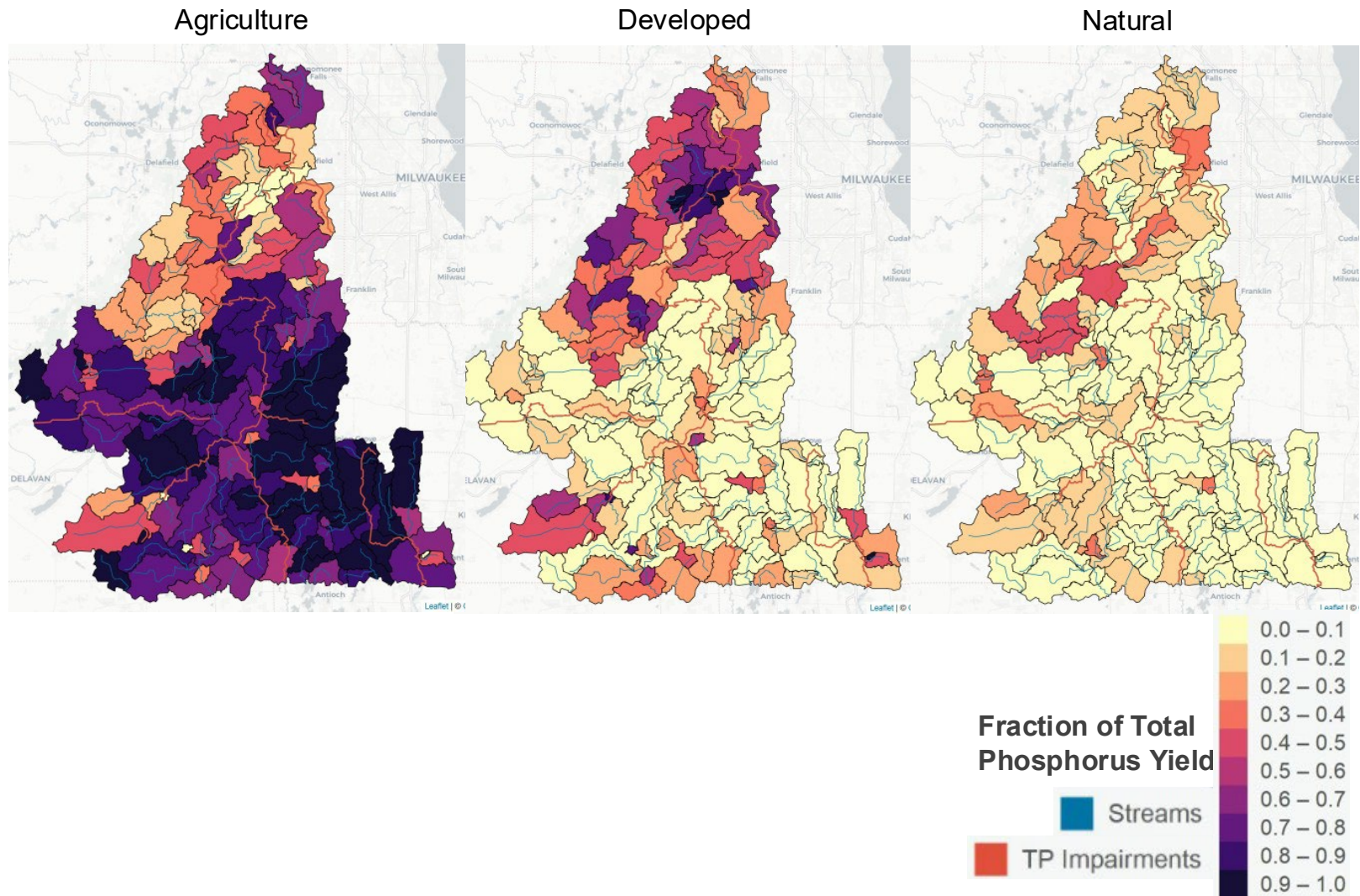
FIGURE I.17 Fraction of Total Watershed Phosphorus Yield by Land Use Categories
