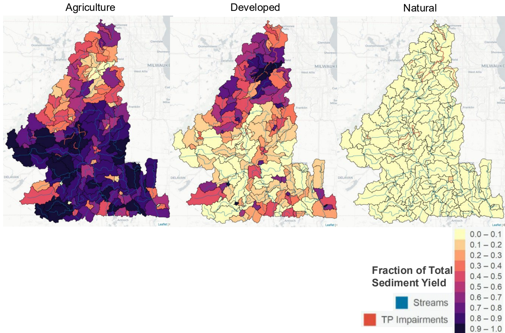
FIGURE I.8 Fraction of Total Watershed Sediment Yield by Land Use Categories
