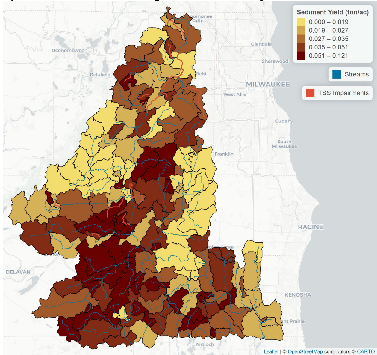
FIGURE I.3 Spatial Distribution of Average Sediment Yield by Model Watershed
