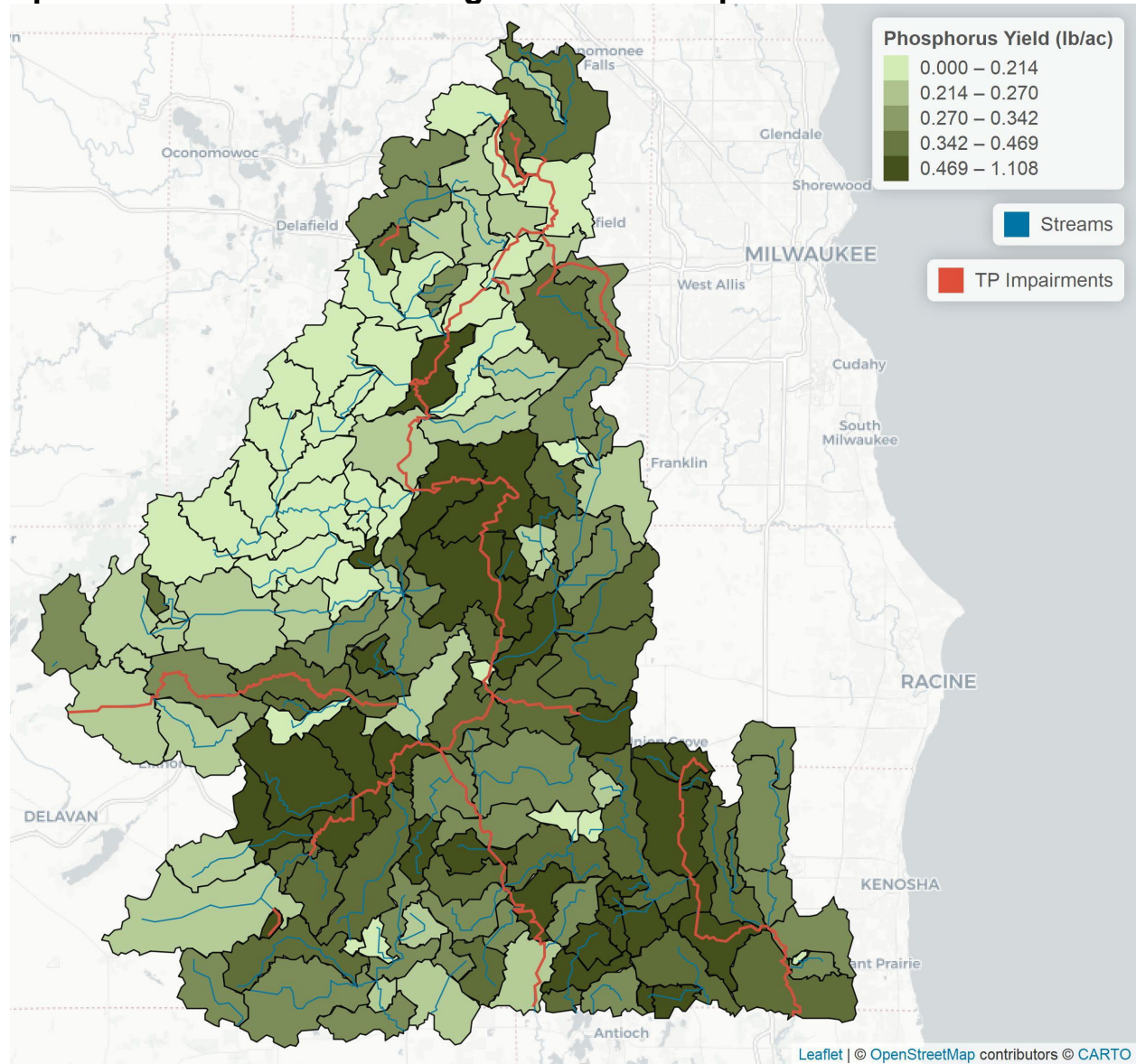
FIGURE 7.2 Spatial Distribution of Average Annual Phosphorus Yield
