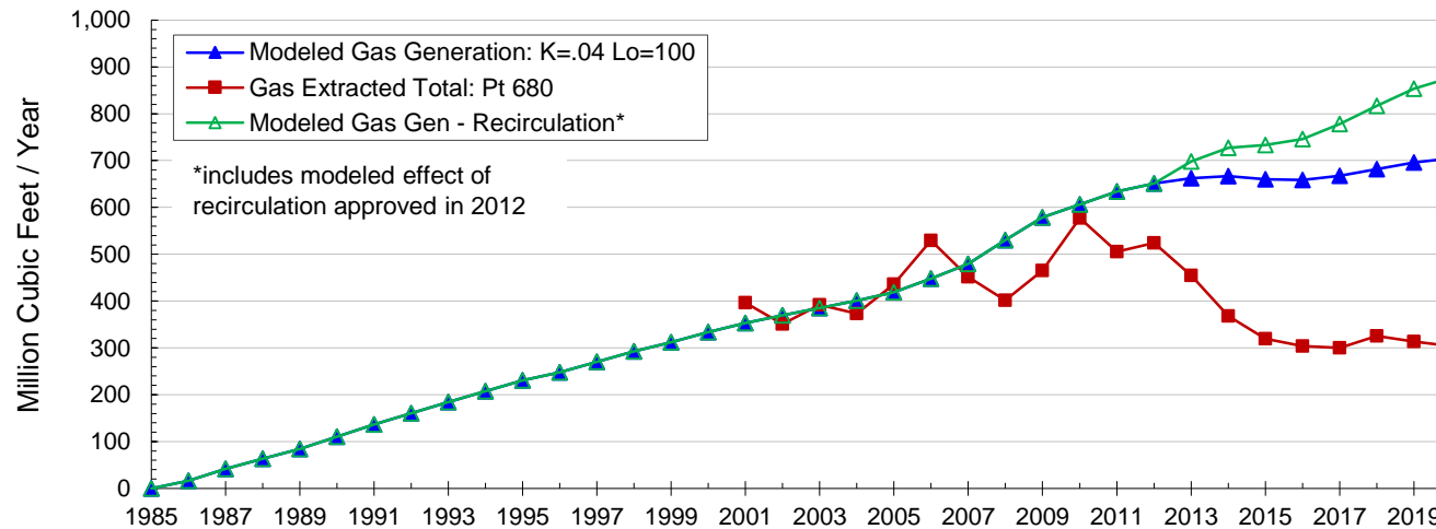
City of Janesville Landfill Lic. Nos 3023 & 3939: Modeled Landfill Gas Generation & Measured Extraction to 2020
