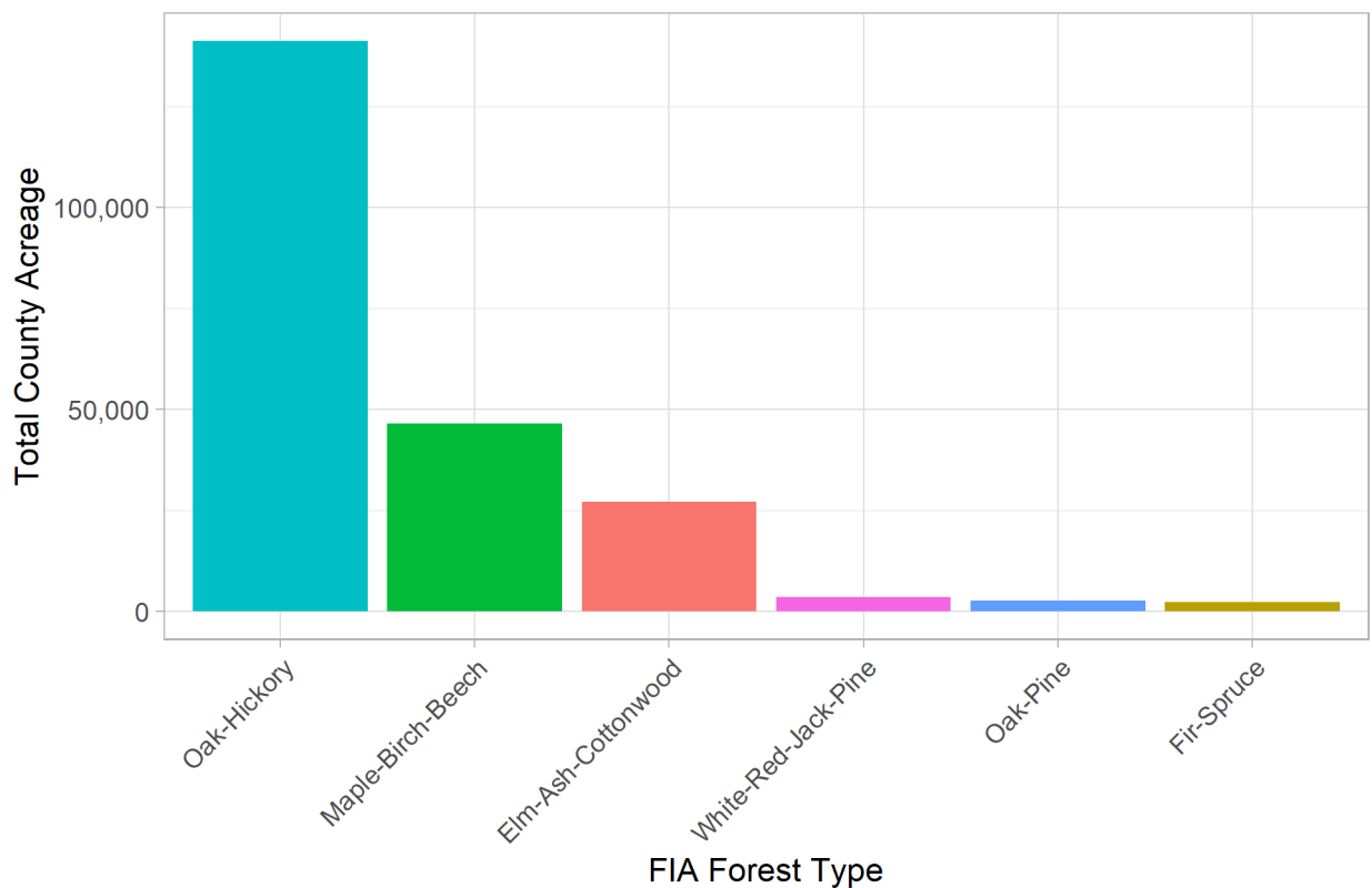
FIA Forest Type Acres in Vernon
