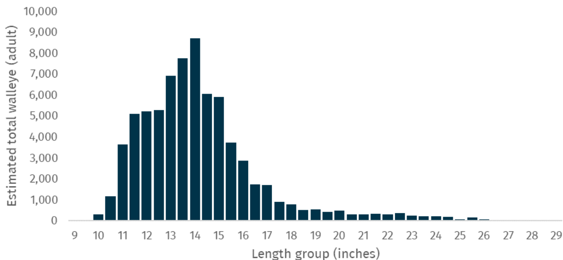
Figure 14. Length frequency of adult walleye estimated to be in the Chippewa Flowage in 2022, based on a whole-lake mark-recapture survey.
