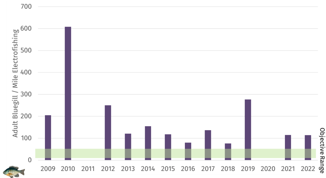
Figure 24. Bluegill relative abundance in the Chippewa Flowage from 2009-2022 late spring electrofishing surveys. No survey data were available in 2011 and 2020. Green shaded area represents the objective range for relative abundance (25-50 per mile electrofished) in the Chippewa Flowage Fisheries Management Plan (2007).
