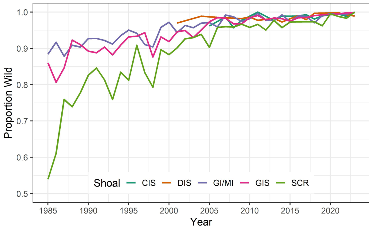
Figure 4. Time series of the proportion of wild (non-hatchery origin) lake trout among five Apostle Islands spawning shoals from 1985 to 2023.
