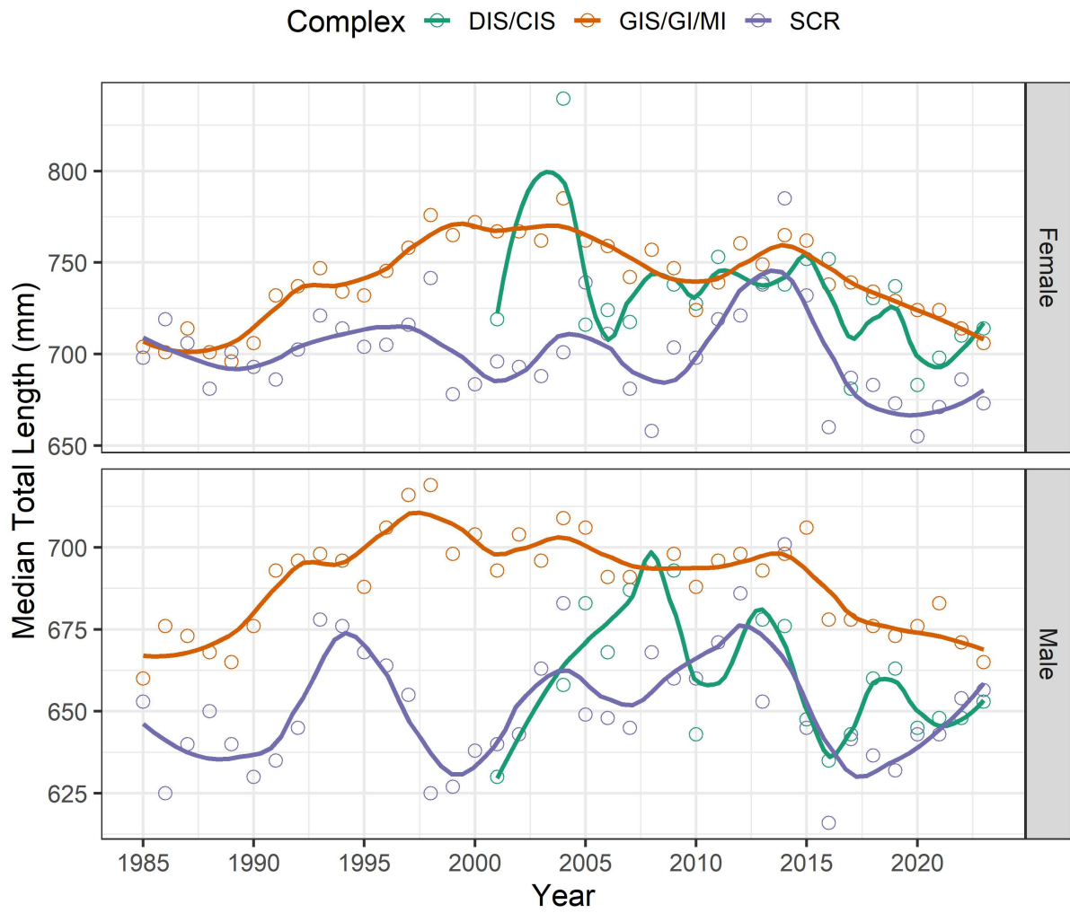
Figure 3. Time series of wild female (top) and male (bottom) lake trout median total length (mm) captured on three Apostle Islands spawning complexes from 1985 to 2023. Trend lines were fit using loess regression. Note the differing y-axis scales between panels.
