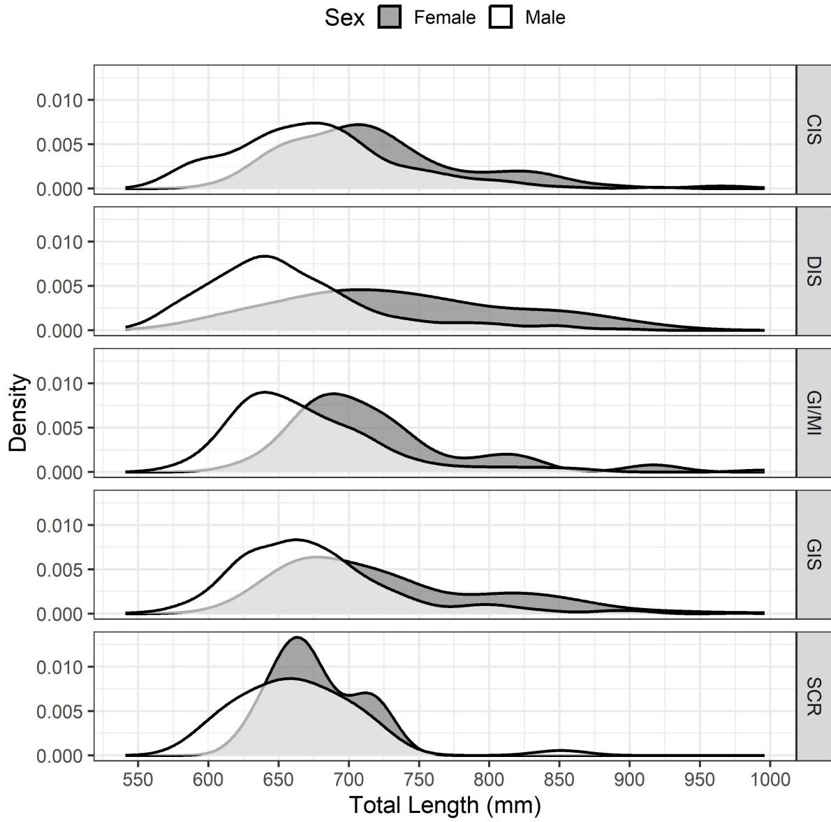
Figure 2. Density plots of male (white) and female (grey) lake trout total lengths on five Apostle Islands spawning shoals in 2023.
