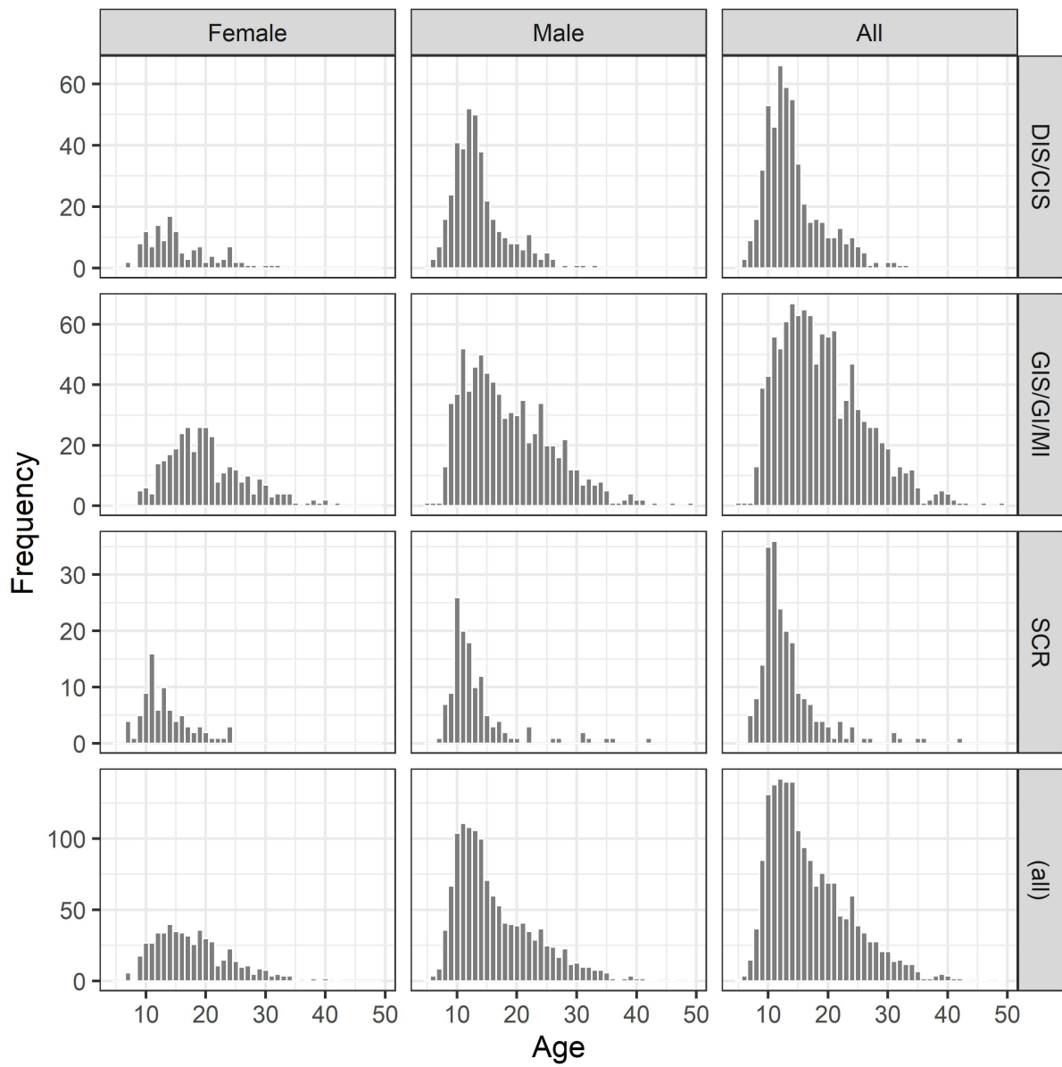
Figure 5. Age frequency plots for male, female and all sexes of lake trout combined that were captured among three Apostle Islands spawning complexes. Data include age estimates from the Fall Lake Trout Survey from 2011 to 2023. Note the differing y-axis scales among panels.
