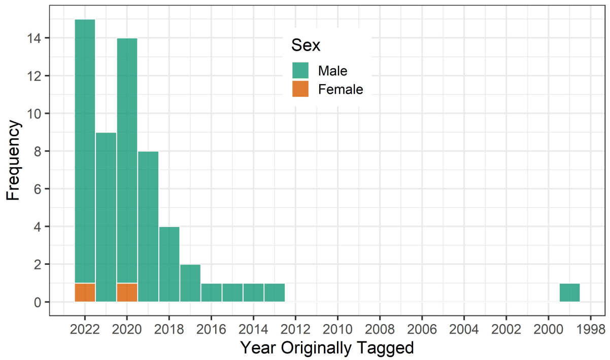
Figure 6. Frequency of fish captured in the 2023 Fall Lake Trout Survey per year the fish was originally tagged (male = green, female = orange).
