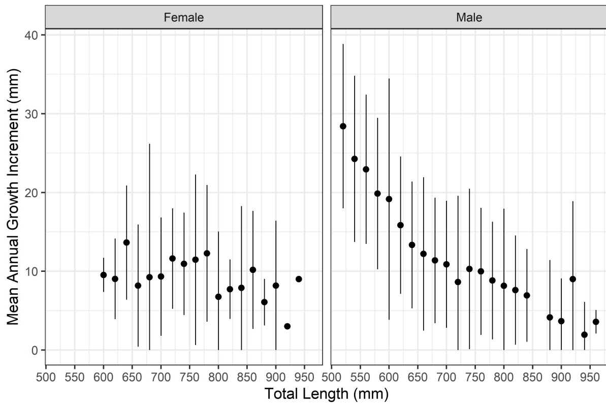
Figure 9. Mean annual growth increment (millimeters) of female (left) and male (right) recaptured wild lake trout during the Fall Lake Trout Survey using data from 2000 to 2023. Vertical bars represent +/- one standard deviation. Individual lake trout were grouped into 20 millimeters length bins based on the observed total length at the most recent capture. Growth increment was computed as the difference between the observed total length and the total length at the most recent capture event divided by the number of years since the most recent capture event.
