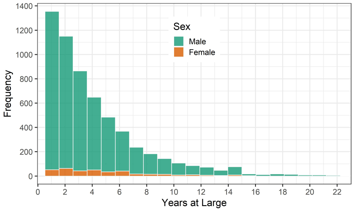
Figure 7. Frequency of the number of years at large since the most recent capture event for all individual recaptured lake trout during the Fall Lake Trout Survey from 1990 to 2023 with males in green and females in orange.
