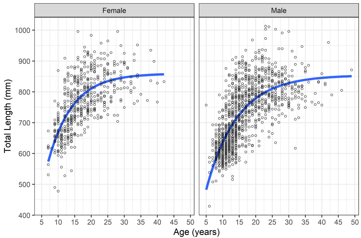
Figure 10. von Bertalanffy growth functions of both female (left) and male (right) lake trout from the Fall Lake Trout Survey from 2011 to 2021.
