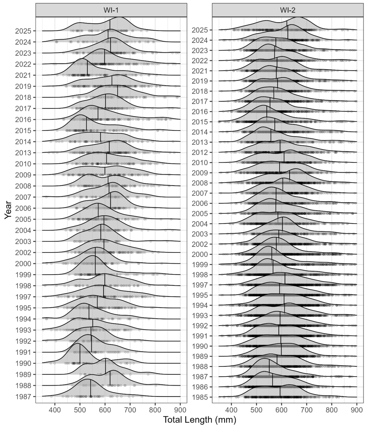
Figure 5. Time series of wild lean lake trout length frequencies in WI-1 (left) and WI-2 (right) waters of Lake Superior from 1985 to 2025. Vertical lines represent the median total length sampled each year.
