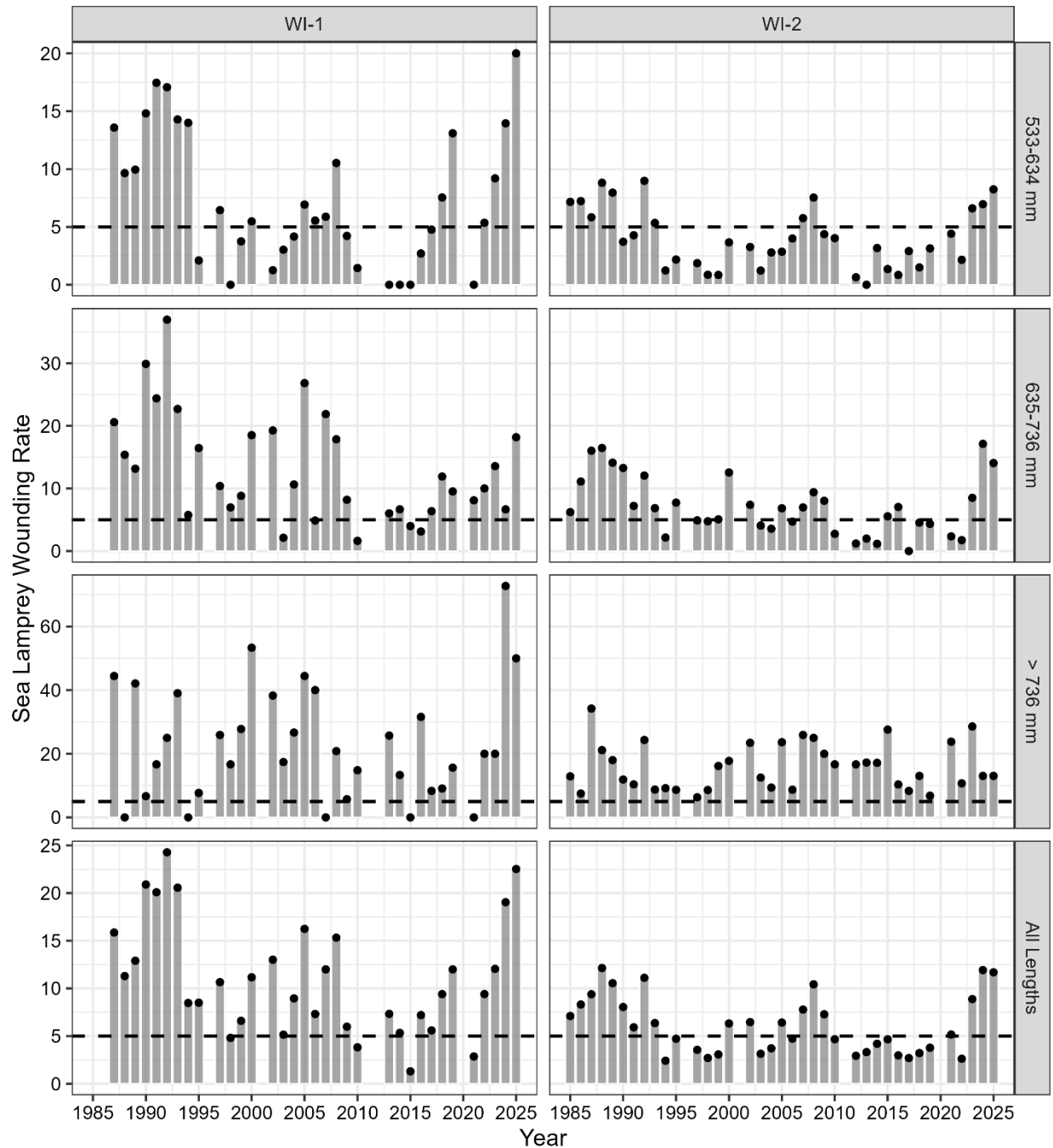
Figure 8. Sea lamprey wounding rates of wild lean lake trout in WI-1 (left) and WI-2 (right) waters of Lake Superior from 1985 to 2025. Wounding rates are represented as the number of A-1 through A-3 type wounds per 100 fish (King 1980; Eshenroder and Koonce 1984). Wounding rates are grouped by total length (LSTC Protocol), and the wounding rate for all fish combined ( \geq 533 mm) is shown on the bottom panel. The LSTC benchmark wounding rate of 5 wounds per 100 fish is represented by the dotted line. Wounding rates are used to estimate potential sea lamprey induced mortality rates of lean lake trout and provide indicators for the GLFC Sea Lamprey Control Program.
