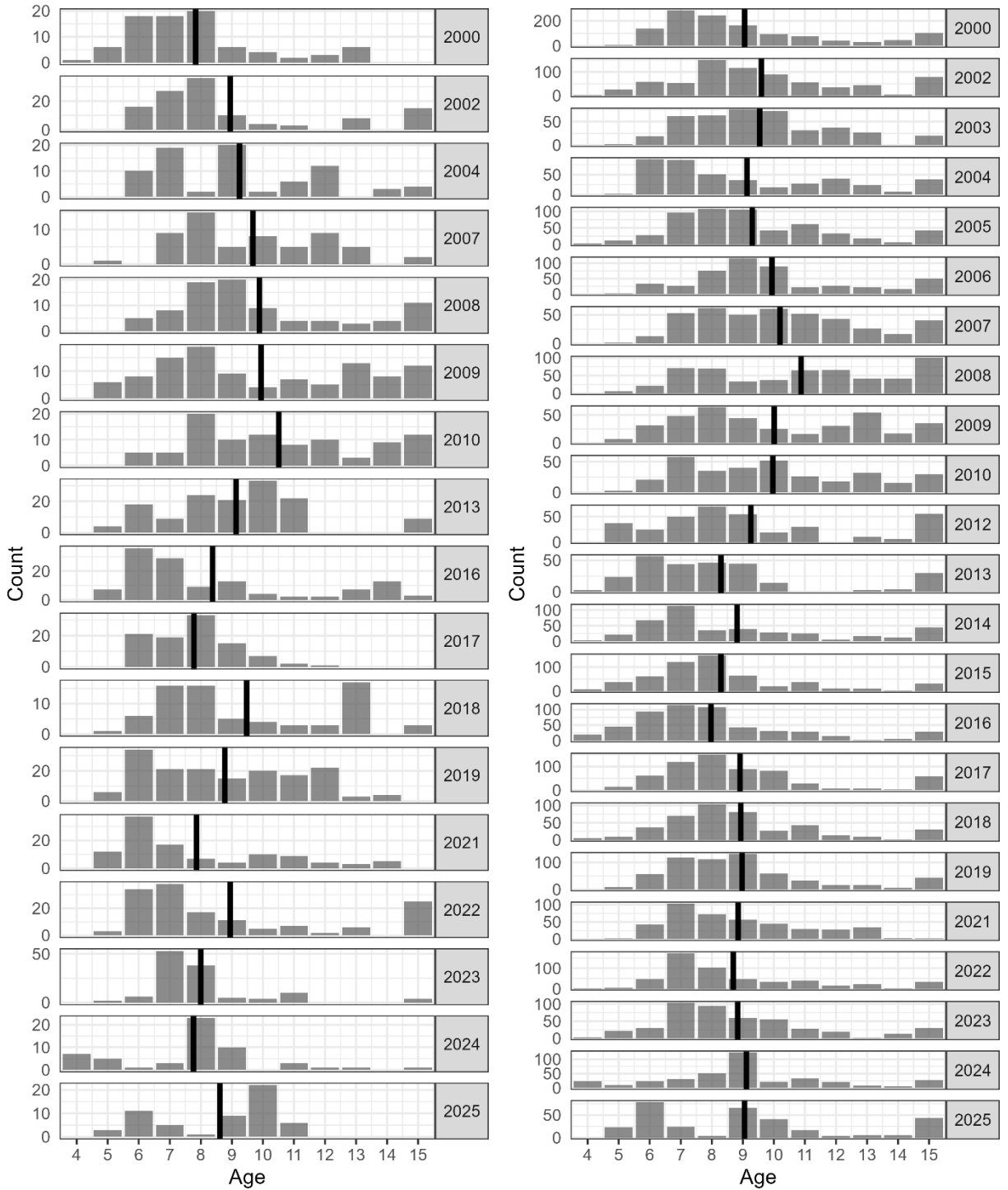
Figure 6. Time series of wild lean lake trout age frequencies in WI-1 (left) and WI-2 (right) waters of Lake Superior from 2000 to 2025. Black vertical lines represent mean annual ages. Age 15 represents a combined group of all ages 15 and up (i.e., 15+).
