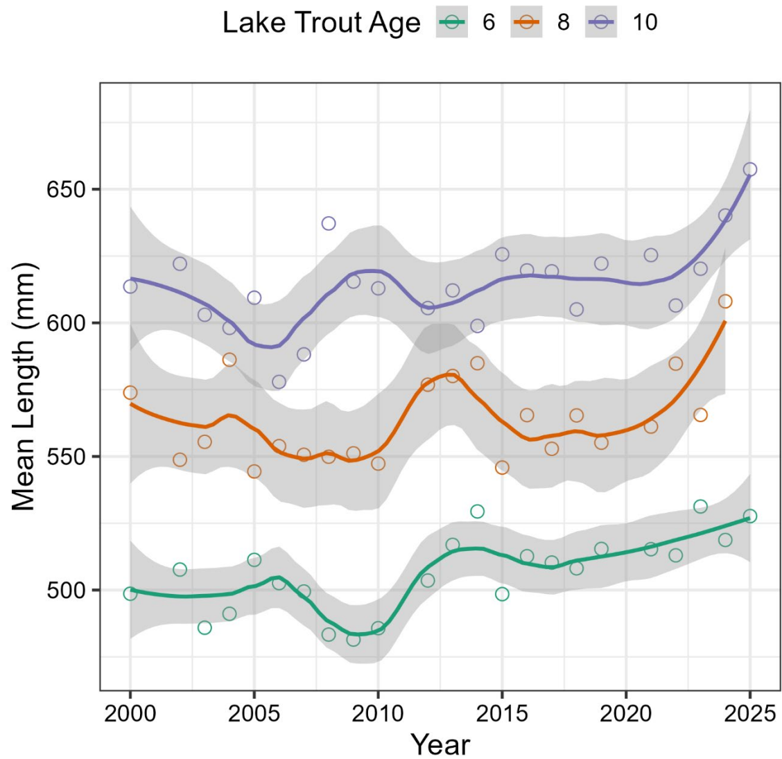
Figure 7. Mean length of age-6 (green), age-8 (orange) and age-10 (purple) wild lean lake trout in WI-2 waters of Lake Superior from 2000 to 2025.
