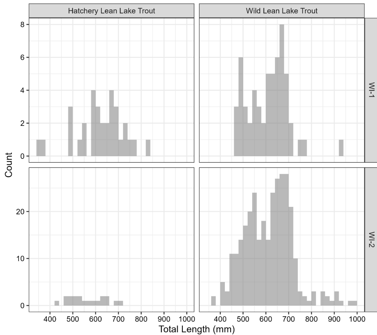
Figure 4. Length frequency histograms of hatchery-origin (left) and wild (right) lean lake trout in WI-1 (top) and WI-2 (bottom) waters of Lake Superior during the 2025 spring survey.
