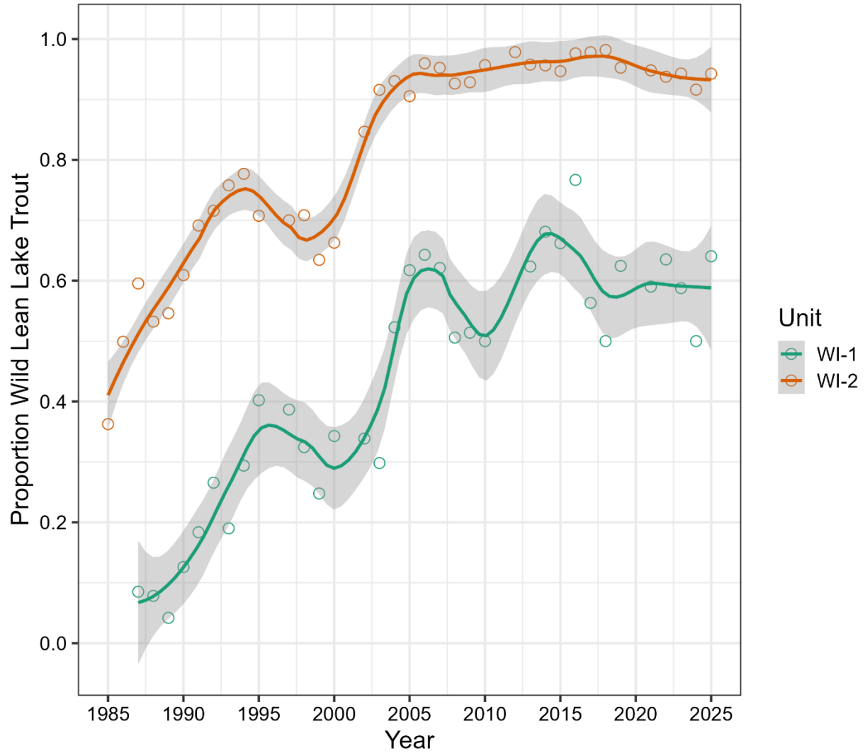
Figure 2. Proportion of lean lake trout catch which was wild (non-hatchery origin) determined by presence of fin clips on hatchery-origin fish in WI-1 (green) and WI-2 (orange) from 1985 to 2025.
