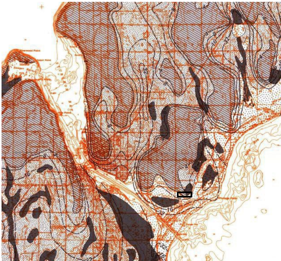
Figure 4 – Depth to Bedrock, excerpted from Geology and Ground Water in Door Cty, WI, with Emphasis on Contamination Potential in the Silurian Dolomite, 1978. Sherrill, M.G. U.S. Geological Survey Water-Supply Paper 2047. Plate 1. Black rectangle indicates the approximate location of Gilbert Farms.
